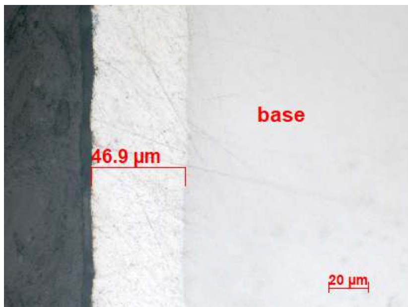
Fig.1 Coating thickness of sample 500×
