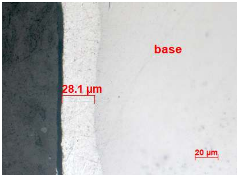
Fig.1 Coating thickness of sample 500×
